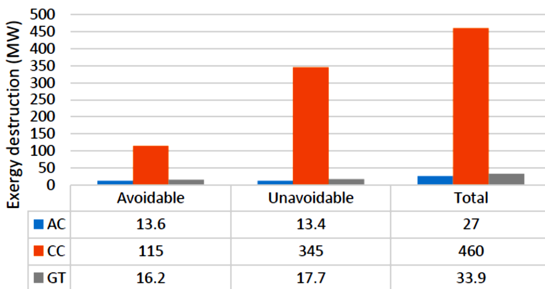
Figure 3: Exergy destruction (MW)
