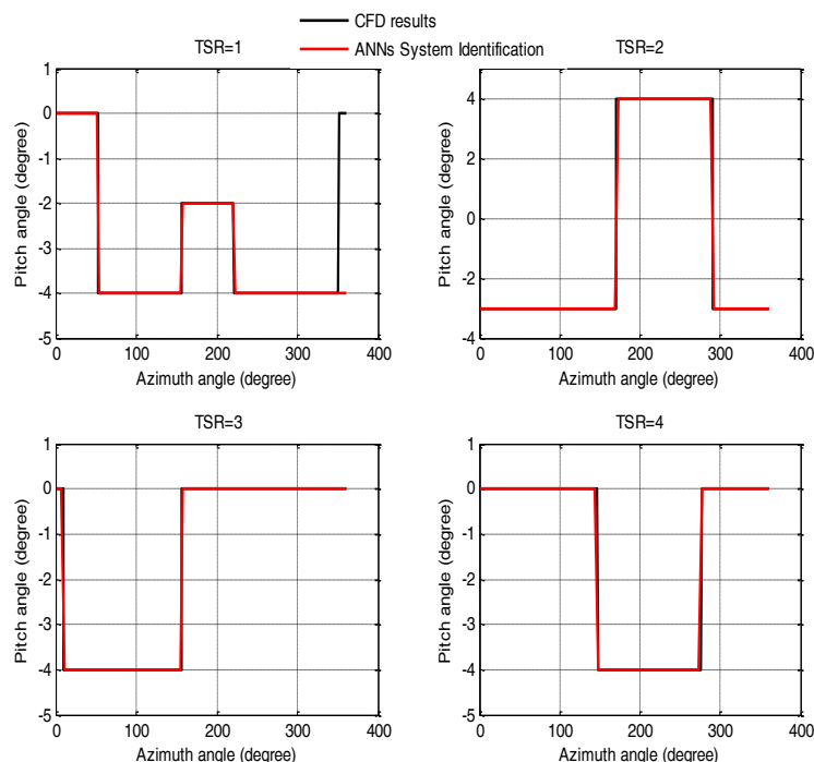
Figure 12: Pitch angle comparisons.
