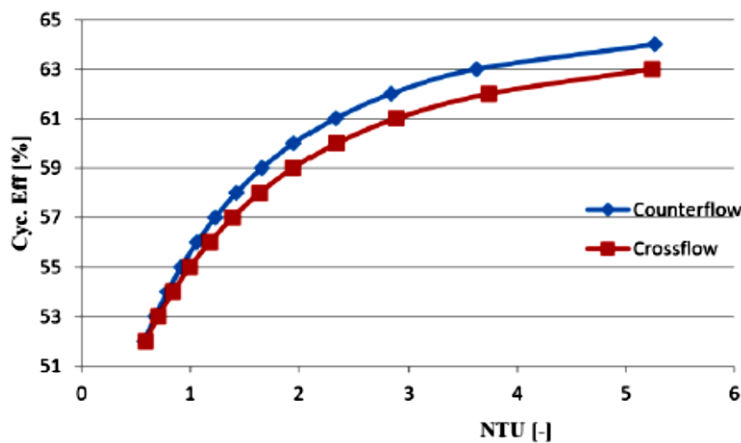
Figure 6: Variation of the Combined Cycle Efficiency with NTU, Plain plate-fin surface 2.0, no intercooler
