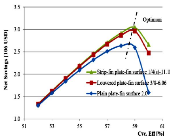
Figure 14: Net Savings with Cycle Efficiency for counter-flow arrangement with no intercooler.
