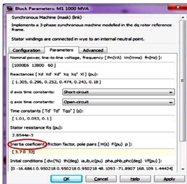
Figure 6: Block Parameters of machine M1
