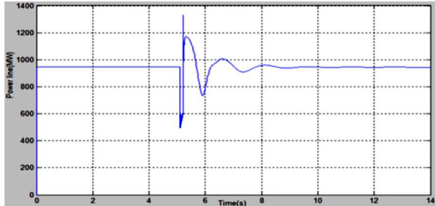
Figure 13: The line power (MW) verses time (s)
