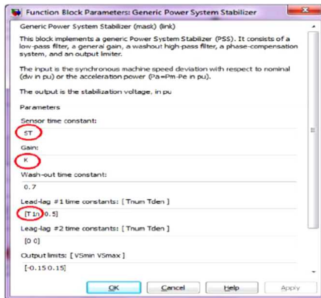
Figure 5: Function Block Parameters: Generic Power System Stabilizer
