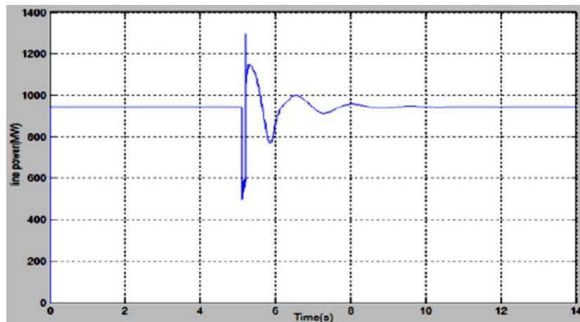
Figure 7: The line power (MW) verses time (s)
