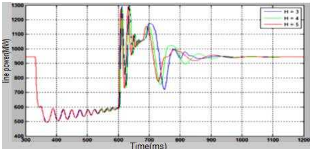
Figure 21: Comparing the line power with using (GA) with (H=3, 4 and 5)
