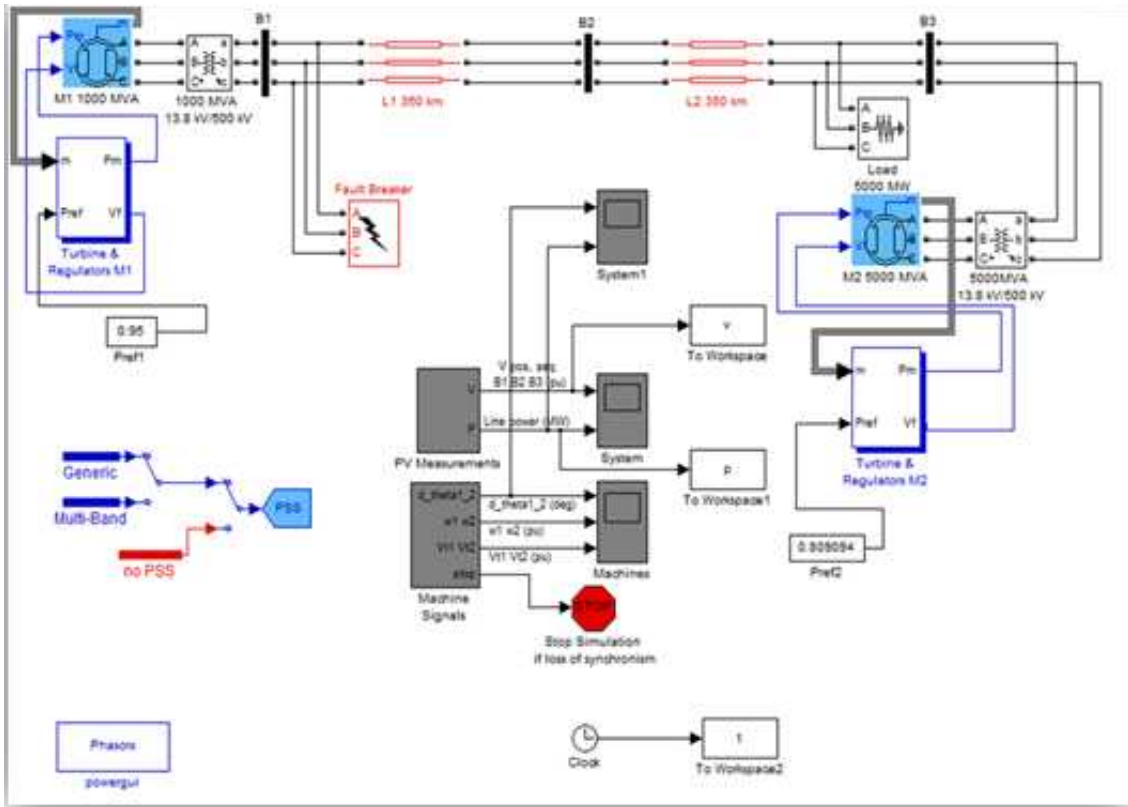
Figure 3: Two-machine transmission system with power system stabilizers (PSS)
