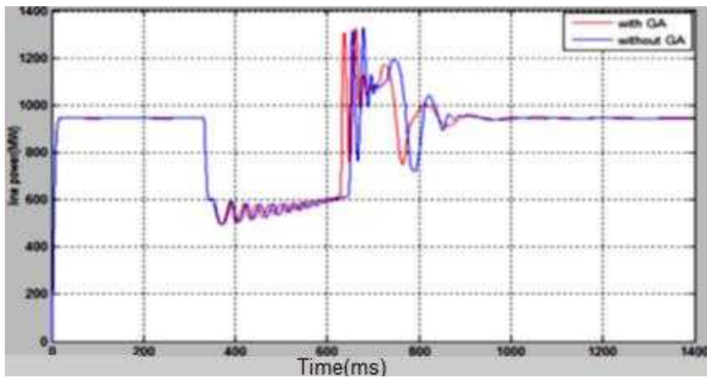
Figure 17: Comparing the line power with and without GA
