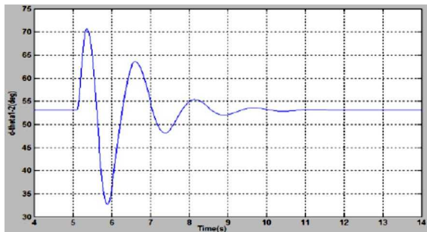
Figure 8: Delta 1-2 (degree) verses time (s)
