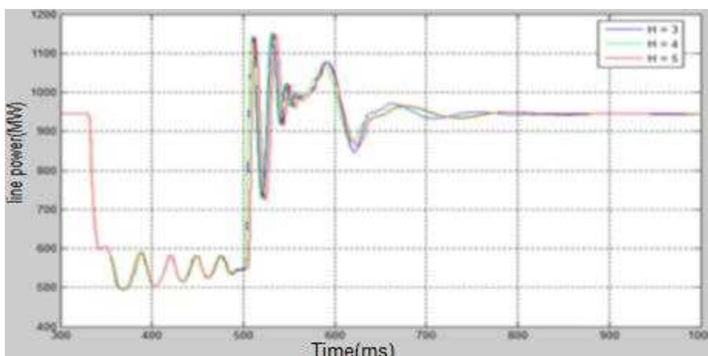
Figure 19: Comparing the line power with using (GA) with ( H=3, 4 and 5 )
