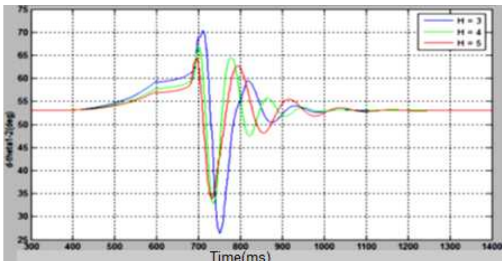
Figure 22: Comparing delta 1-2 with using (GA) with (H=3, 4 and 5)
