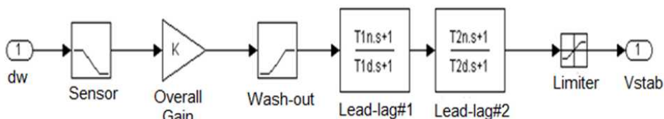
Figure 2: Block diagram of power system stabilizer.
