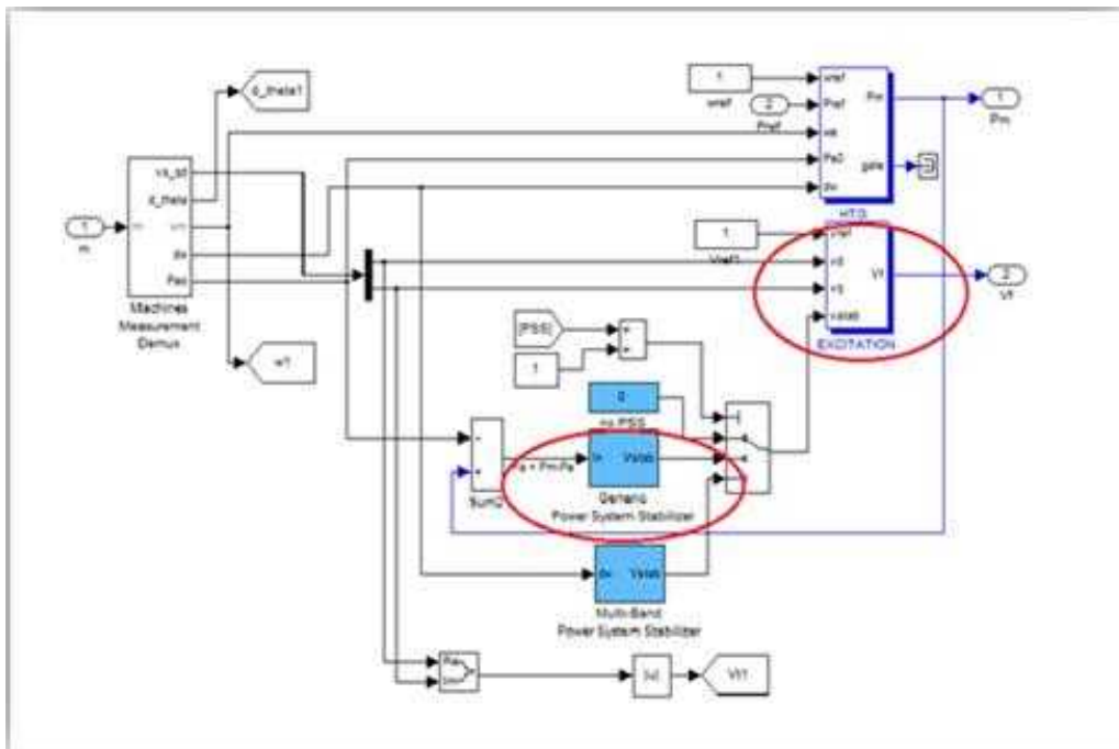
Figure 4: Power system stabilizer with excitation system.
