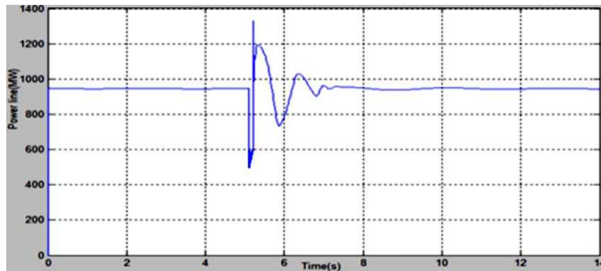
Figure 14: Delta 1-2 (degree) verses time (s)
