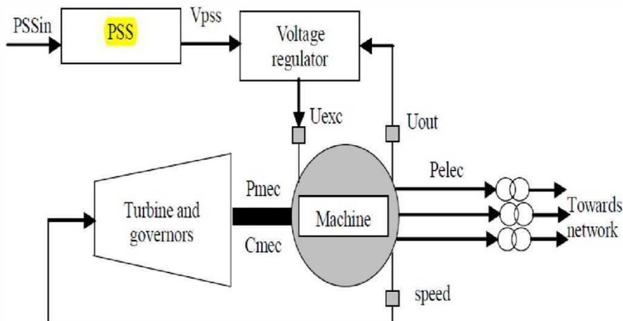
Figure 1: Overall structure of a machine connected to the network.
