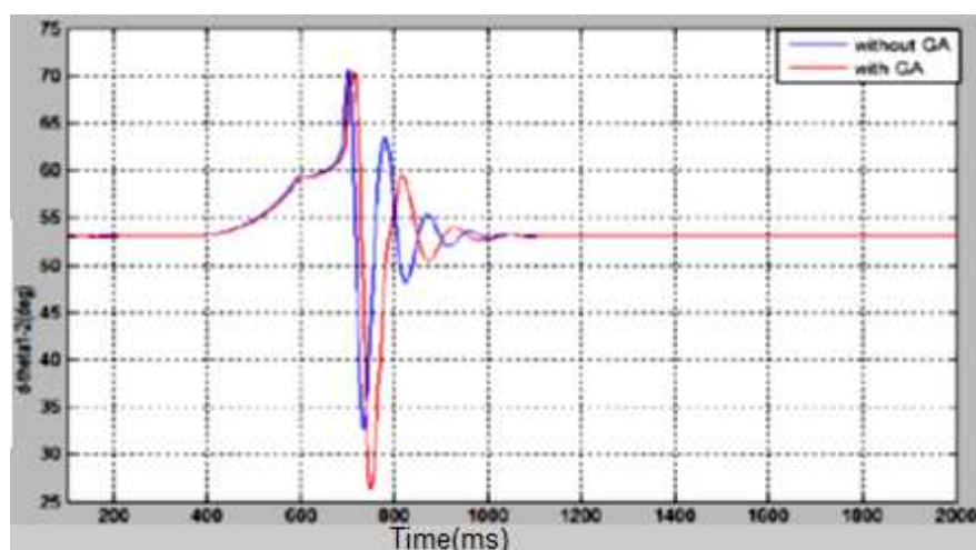
Figure 12: Comparing delta 1-2 with and without GA
